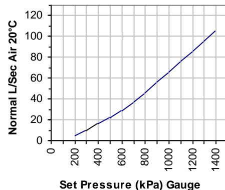
FLOW RATE CHART
